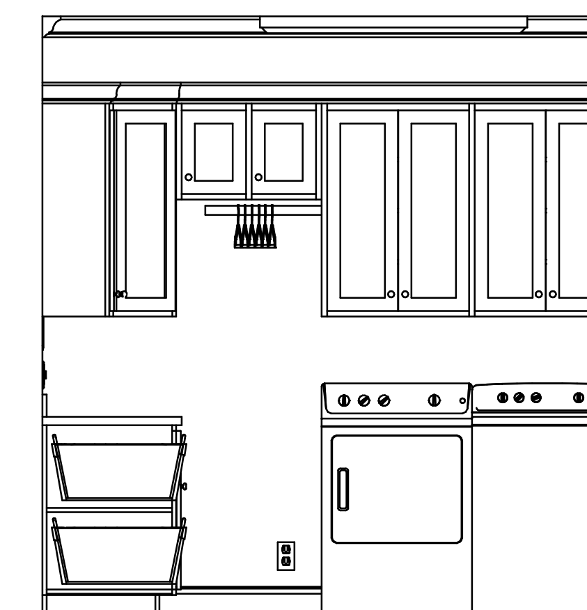
L2 LAUNDRY SCALE: 1/2"=1'
