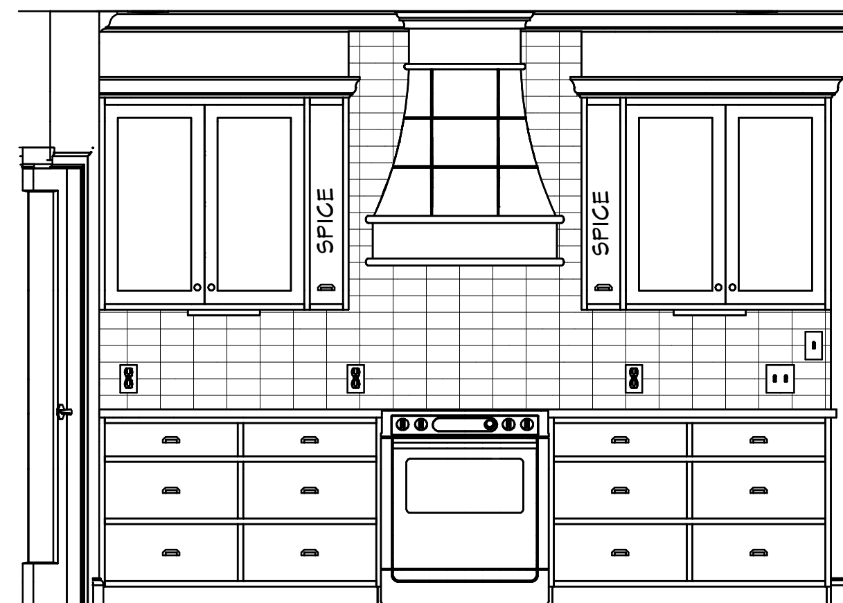
K1 KITCHEN SCALE: 1/2"=1'
